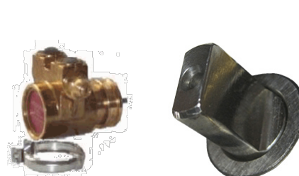
1133004 POMPANTE PROCON BILANCIATO A FASCETTA 160/200 l/h / BALANCED PROCON PUMPING ELEMENT WITH BAND 16/200 l/h 69000002: RANCILIO SPA 26302: CMA MACCHINE PER CAFFE' SRL
