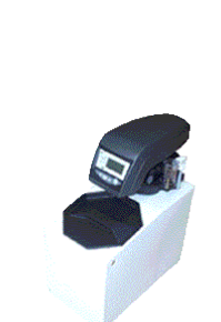
L=230mm, P=440 mm, H=540 mm, TIMER=1112314, KIT TESTATA=6101018, KIT MEMBRANE=6101019
