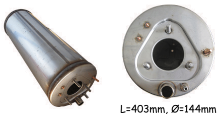
L=403mm, Ø=144mm
