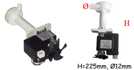
H=225mm, Ø12mm
